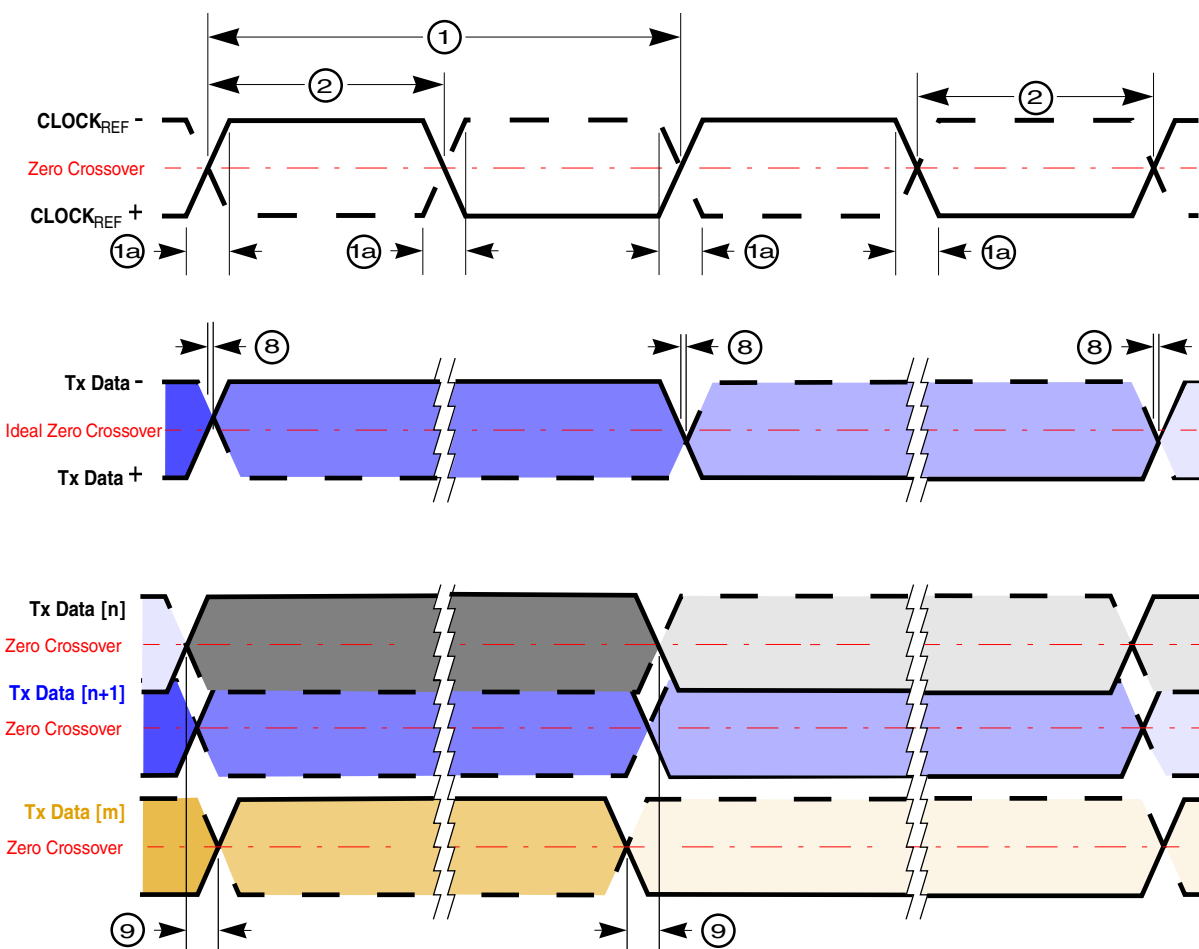
Figure 29. Aurora timings
