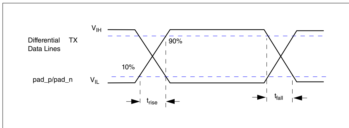
Figure 14. Rise/fall time
