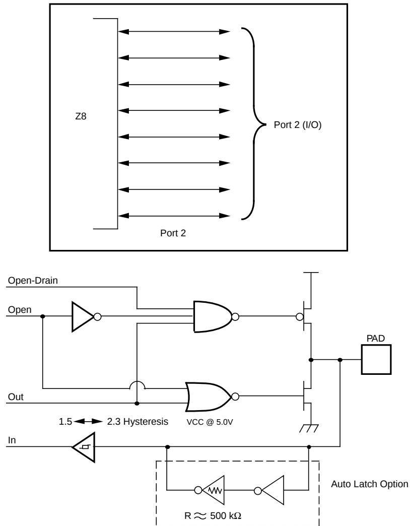
Figure 9. Port 2 Configuration
