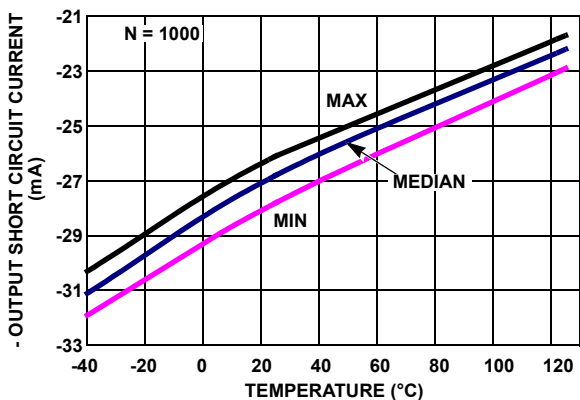
FIGURE 54. ISL28276, ISL28476 - OUTPUT SHORT CIRCUIT CURRENT vs TEMPERATURE, V_{IN} = +2.55V , R_L = 10 , V_+ , V_- = \pm 2.5V
