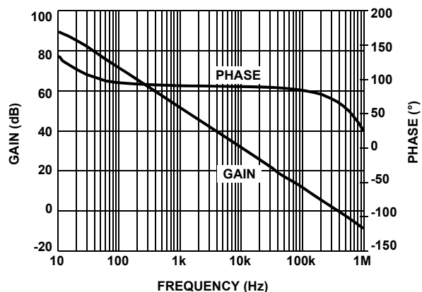
FIGURE 6. A_{VOL} vs FREQUENCY @ 1k \Omega LOAD
