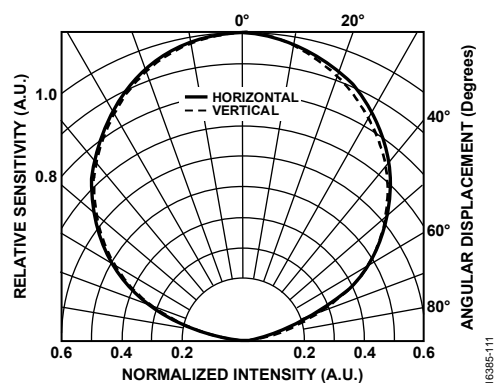
Figure 10. PDET1 Relative Sensitivity vs. Angular Displacement
