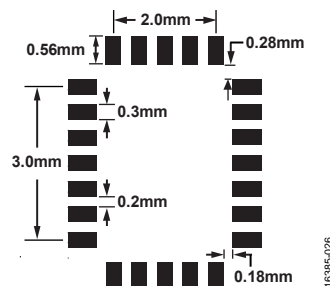
Figure 31. Land Pattern
