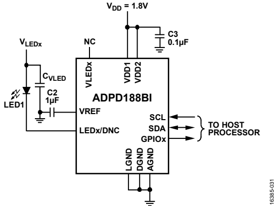
Figure 36. Using the ADPD188BI LED Drivers to Drive External LEDs
