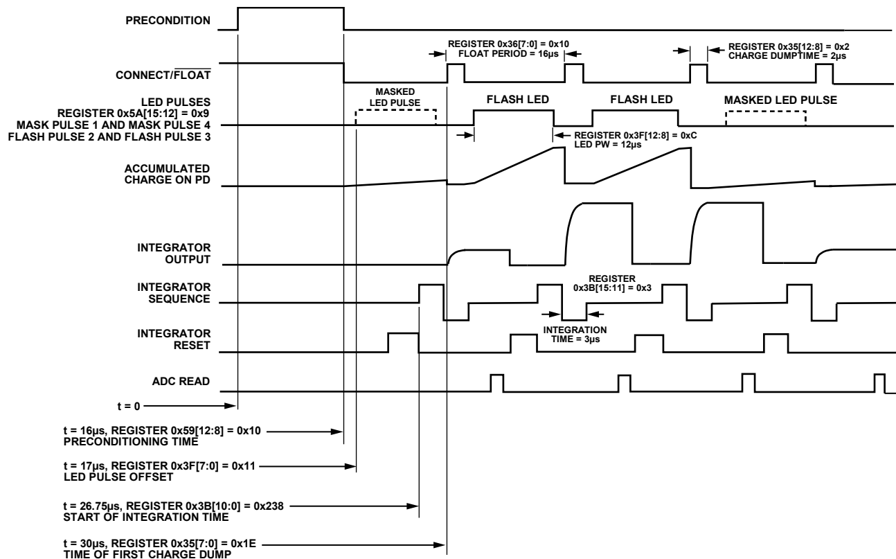
Figure 42. Example Timing Diagram of Four Pulse Float LED Mode Sequence
