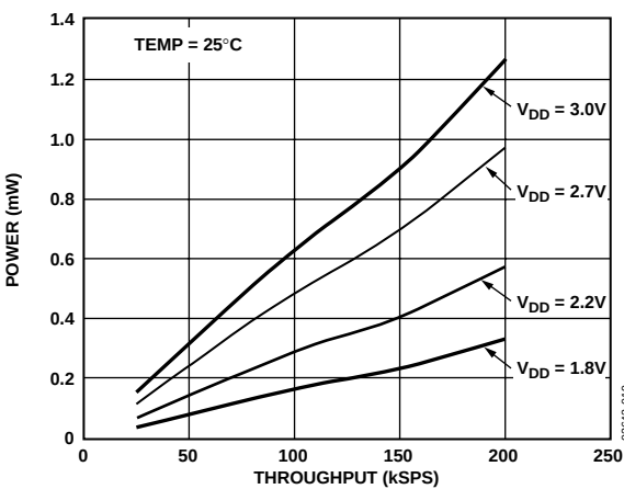
Figure 18. AD7466 Power Consumption vs. Throughput Rate, SCLK 3.4 MHz
