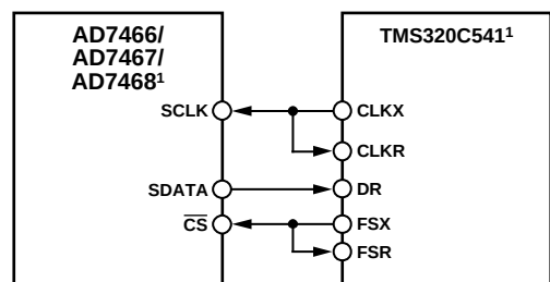
Figure 32. Interfacing to the TMS320C541
