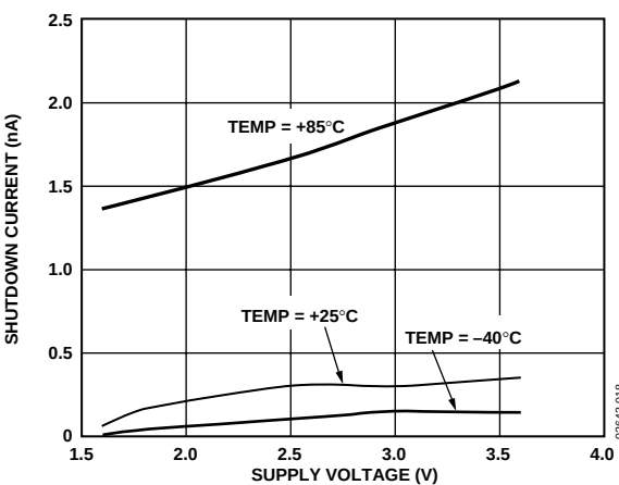
Figure 17. Shutdown Current vs. Supply Voltage
