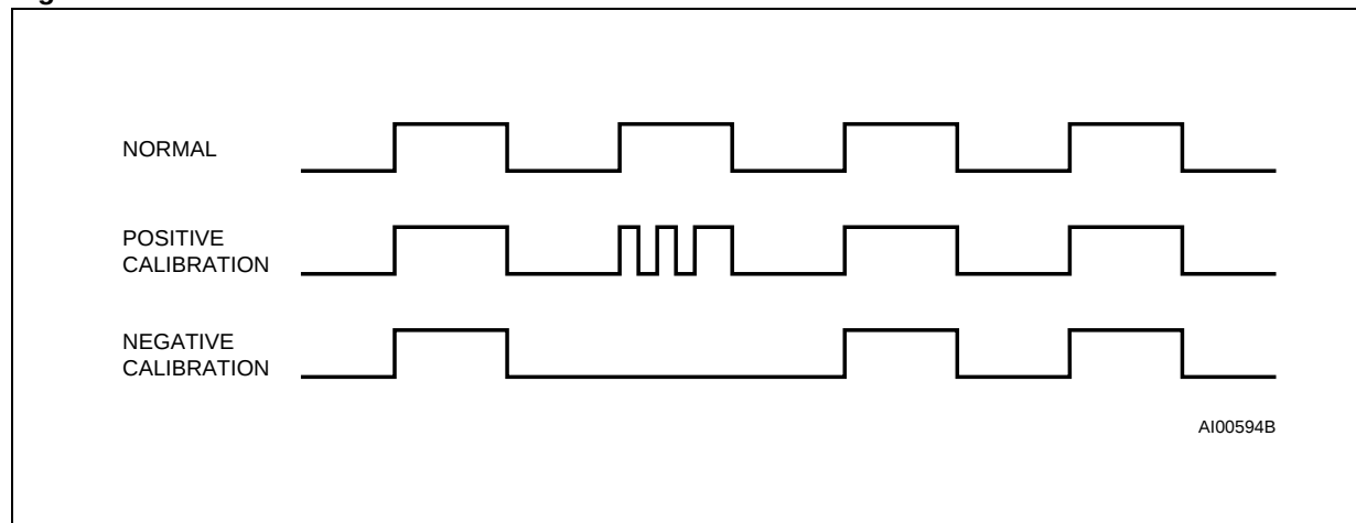
Figure 13. Clock Calibration
