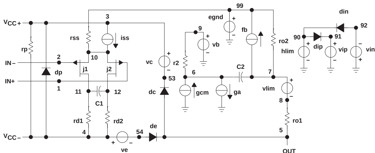
Figure 73. Boyle Subcircuit
