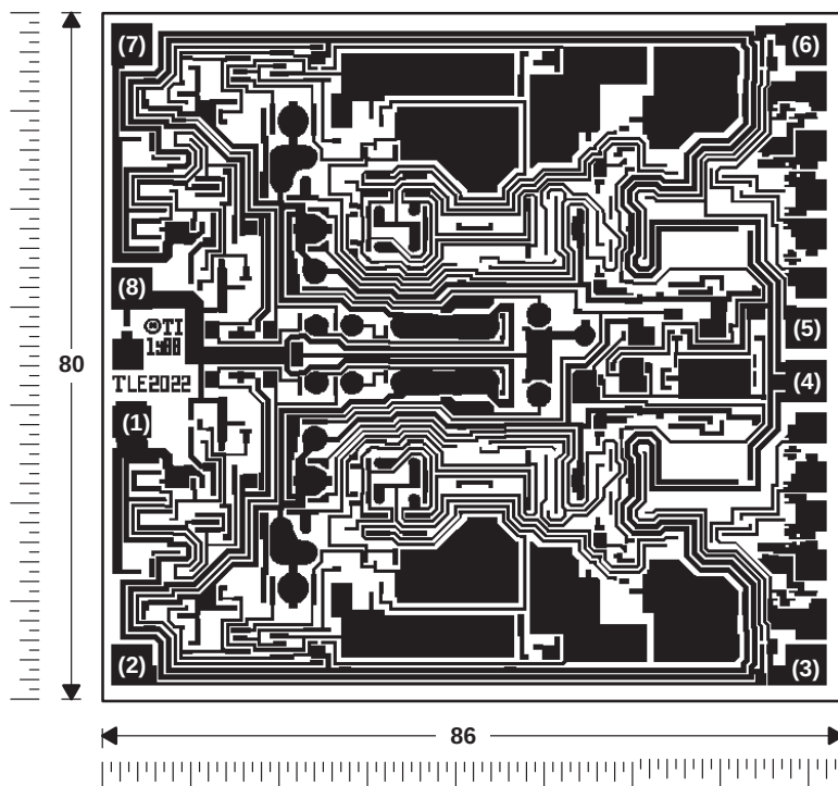
BONDING PAD ASSIGNMENTS
