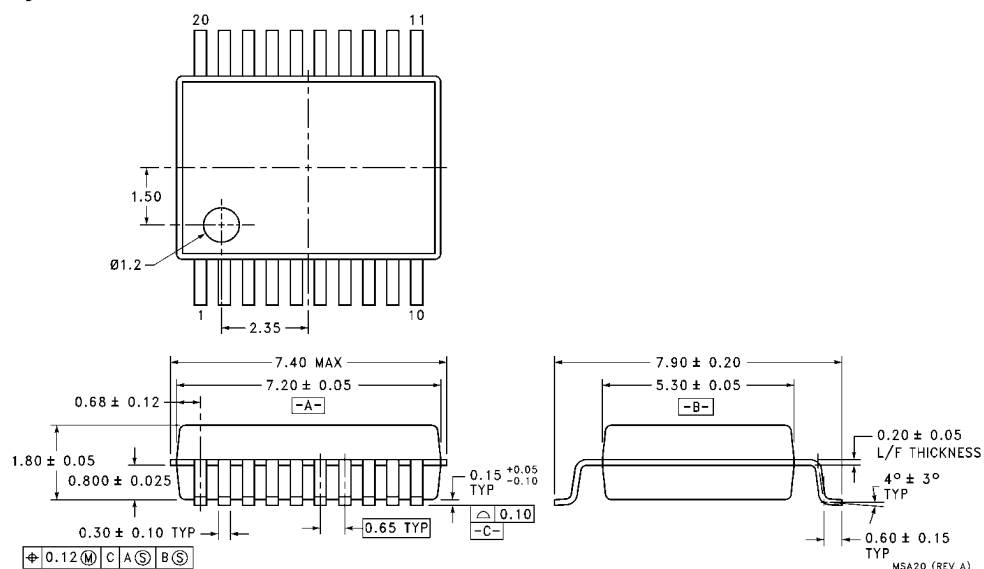
20-Lead Shrink Small Outline Package (SSOP), EIAJ TYPE II, 5.3mm Wide Package Number MSA20
