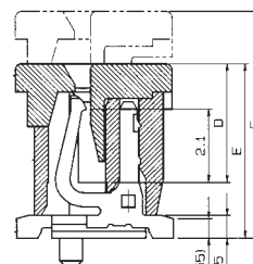
SECT. X-X
