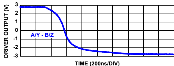
FIGURE 38. ISL32602E, ISL32603E DRIVER AND RECEIVER WAVEFORMS, HIGH TO LOW
