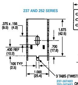
237 AND 252 SERIES Dimensions: in. (mm)
