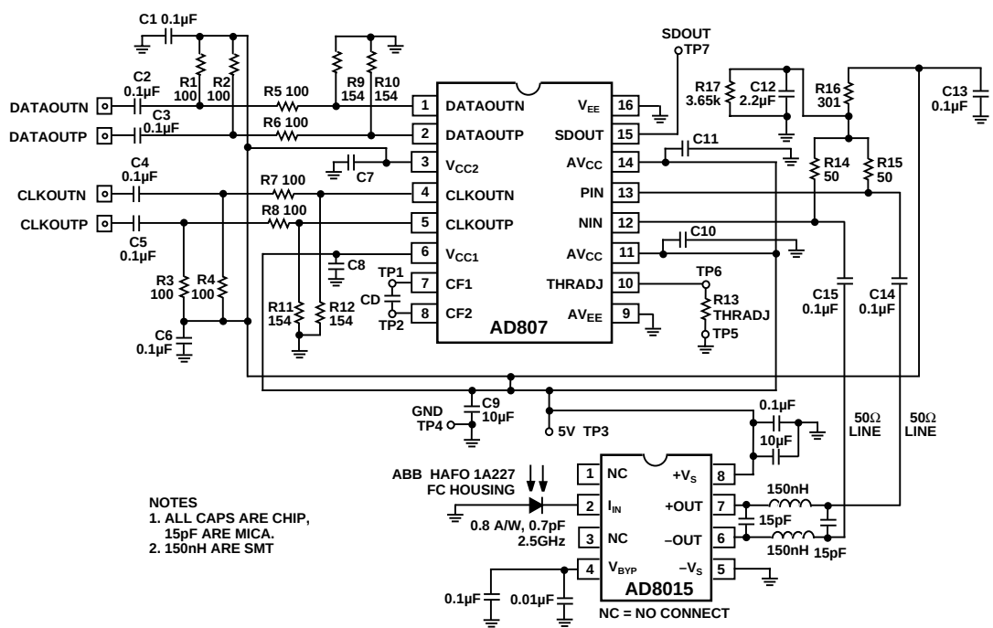
Figure 23. Low Cost 155 Mbps Fiber Optic Receiver Schematic
