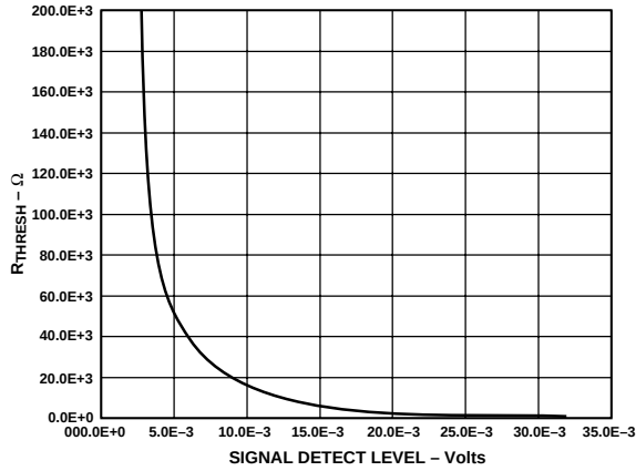
Figure 6. Signal Detect Level vs. R_{THRESH}
