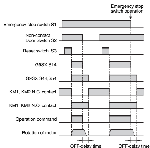
Timing chart
