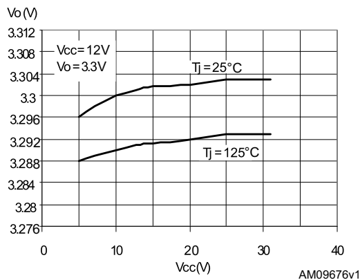
Figure 33. Line regulator
