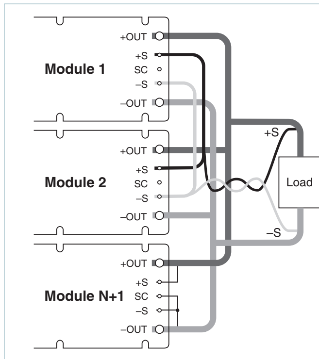
Figure 11 — N+1 module array output connections
