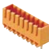
Pin headers SL 3.5/180G
