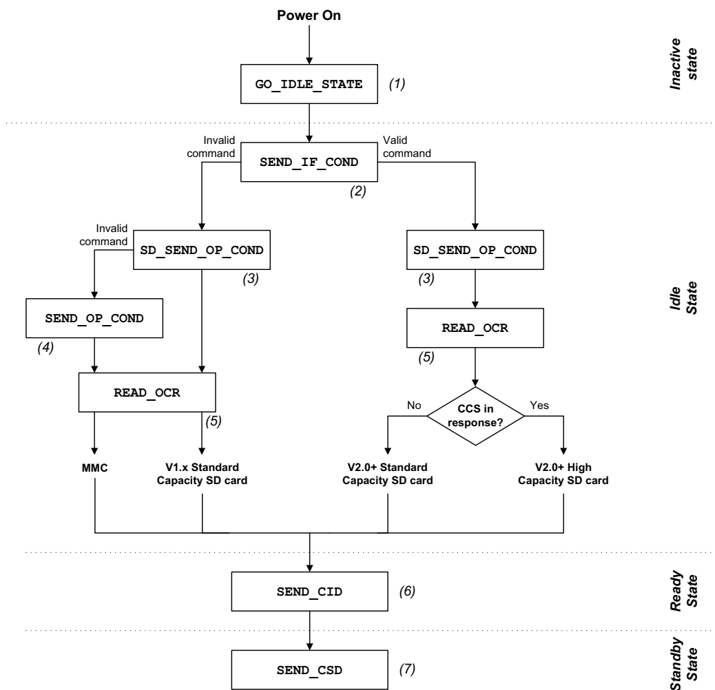
Figure 12-13 Simplified SD/MMC SPI mode initialization and state transitions
