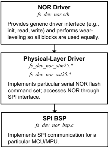
Figure 14-3 NOR driver architecture (serial NOR flash)
