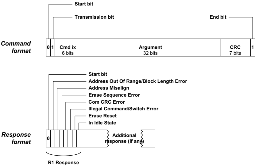
Figure 12-12 SD/MMC SPI mode command and response formats
