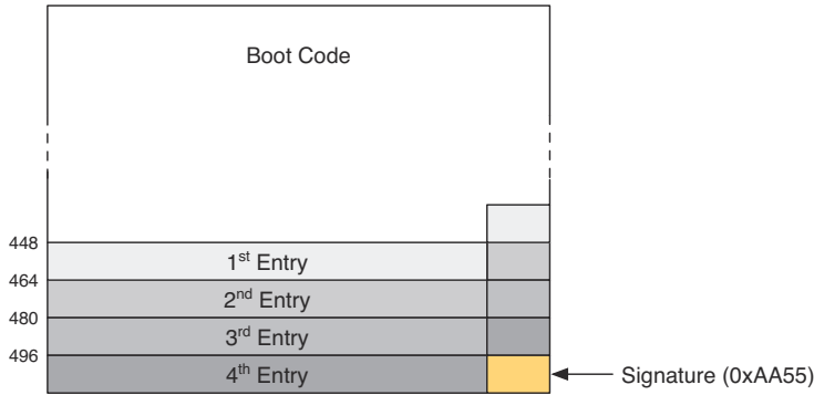
Figure 5-4 Master boot record
