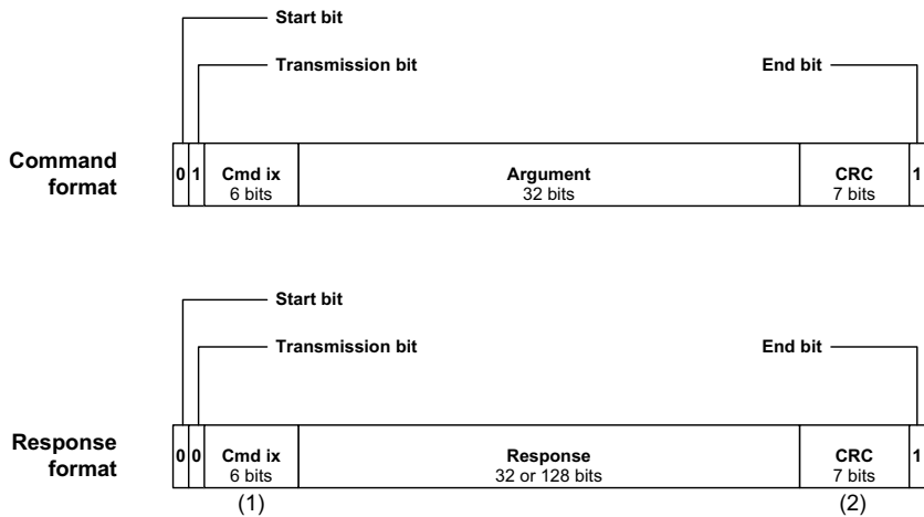
Figure 12-11 SD/MMC SPI mode communication sequence
