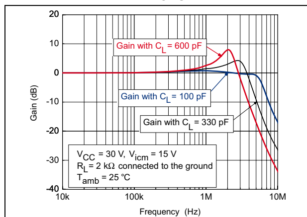
Figure 18. Frequency response for different capacitive loads at V_{CC} = 30\text{ V} , V_{icm} = 15\text{ V} and T = 25\text{ °C}
