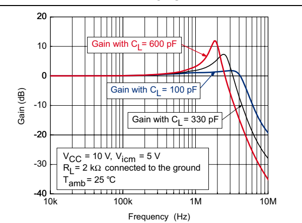
Figure 17. Frequency response for different capacitive loads at V_{CC} = 10\text{ V} , V_{icm} = 5\text{ V} and T = 25\text{ °C}
