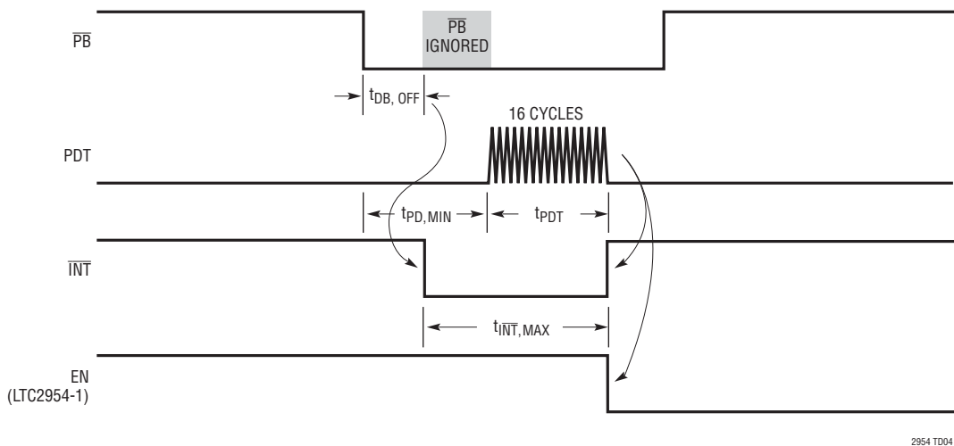
Forced Off, Power-Down Timing, \overline{\text{PB}} Pressed and Held Low for t > (t_{\text{PD, MIN}} + t_{\text{PDT}})
