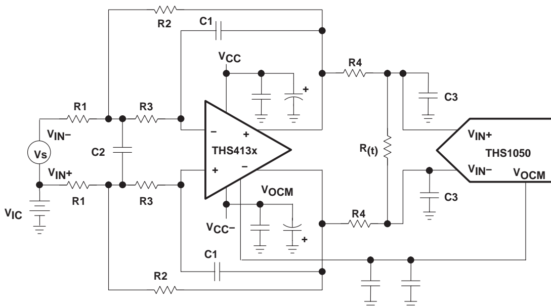
Figure 34. Antialias Filtering
