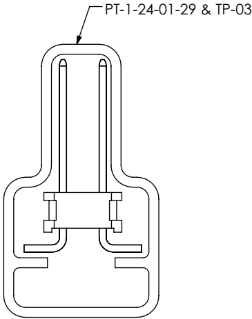
-53 & -54 LEAD STYLES
