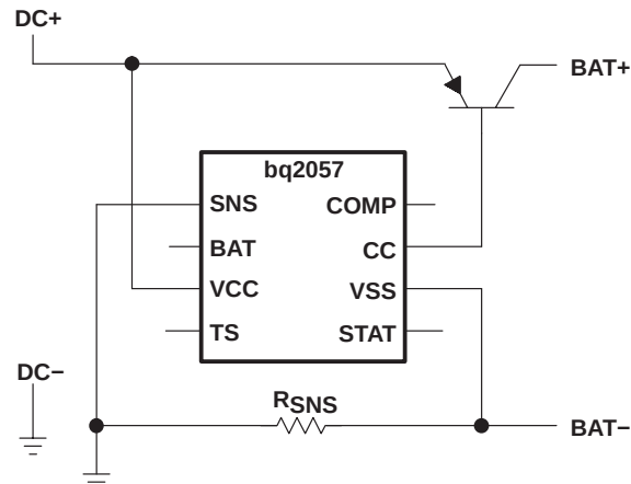
Figure 6. Low-Side Current Sensing
