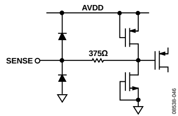
Figure 37. Equivalent SENSE Circuit
