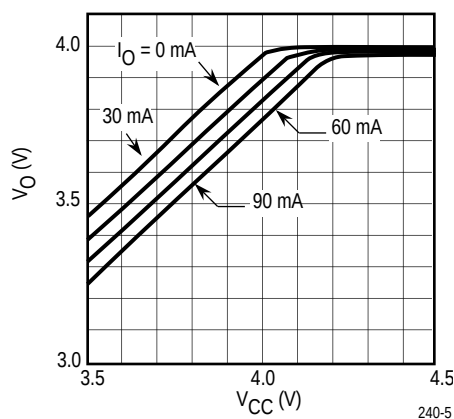
SUPPLY VOLTAGE vs. OUTPUT VOLTAGE
