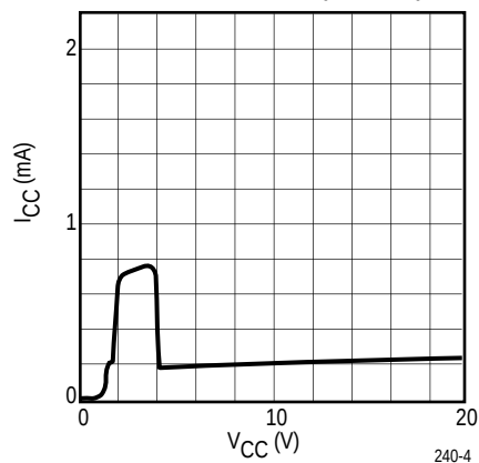
SUPPLY CURRENT vs. INPUT VOLTAGE (NO LOAD)
