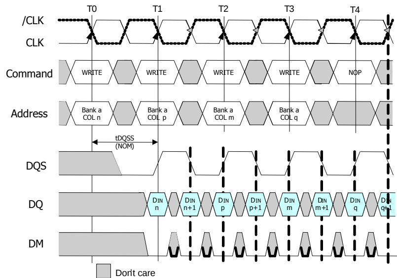
Figure24 : Random Write to write
