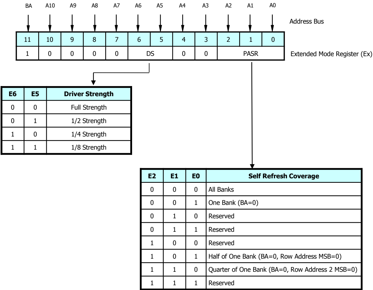
Figure5 : Extended Mode Set (EMRS) Register
