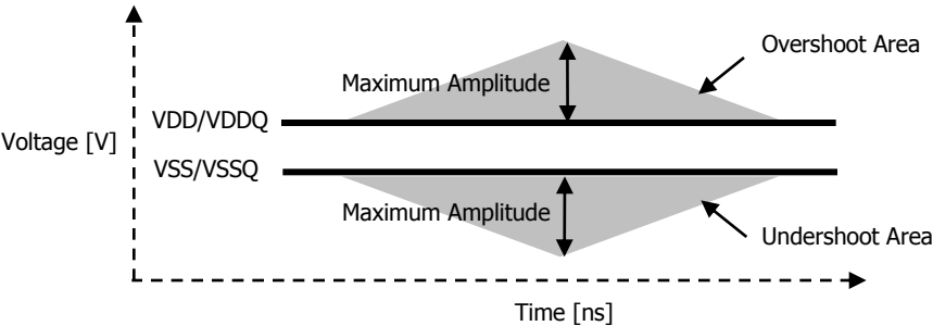
Figure9: AC Overshoot/Undershoot Definition
