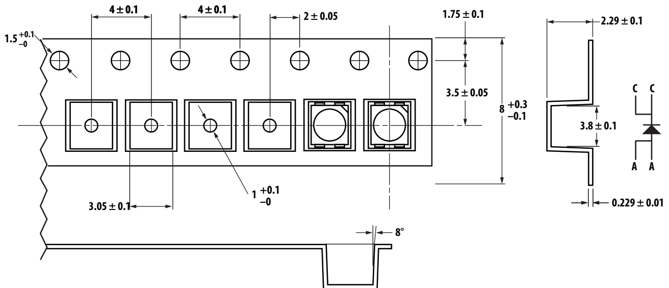
Figure 16. Tape dimensions
