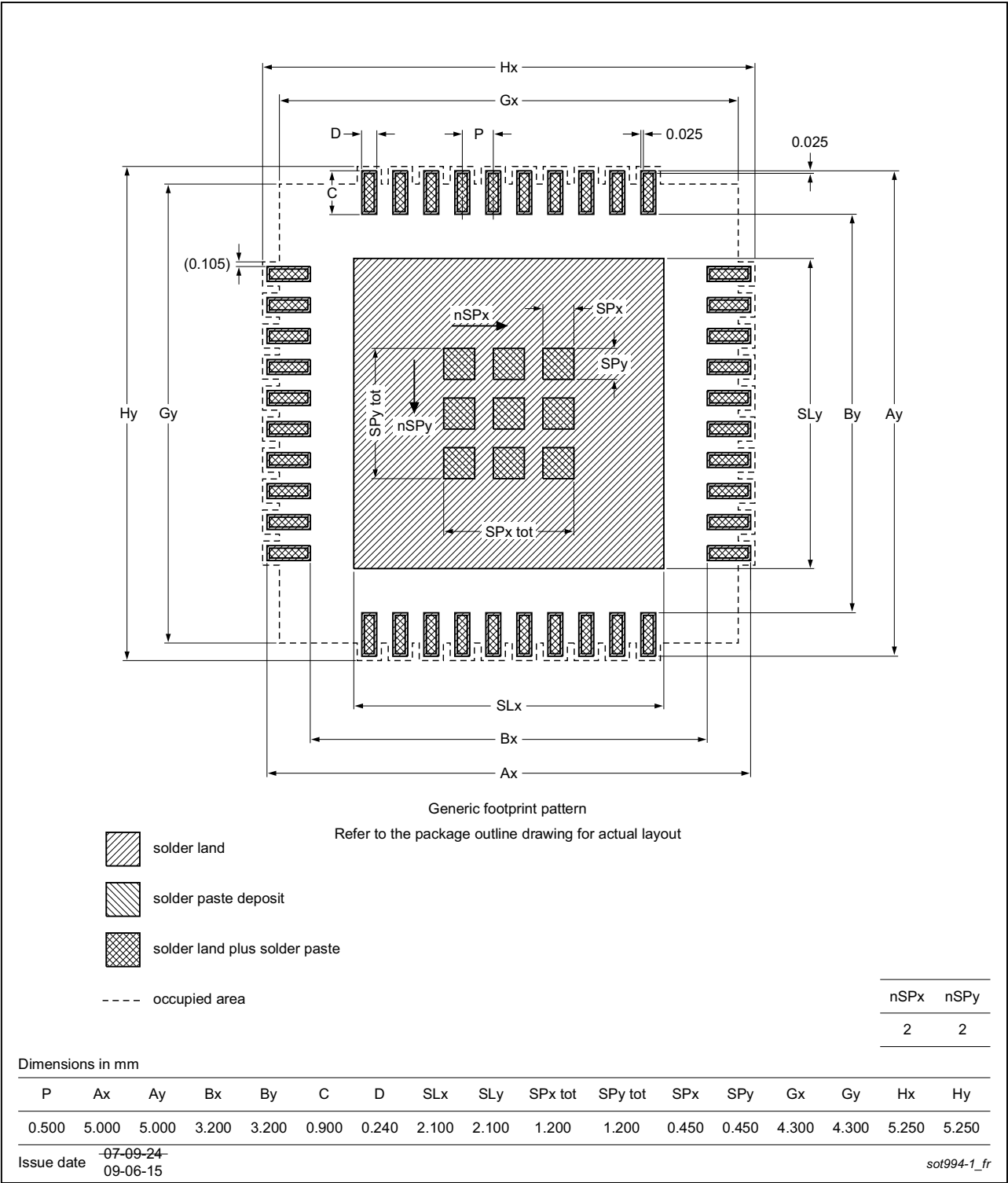
Footprint information for reflow soldering of HVQFN24 package SOT994-1
