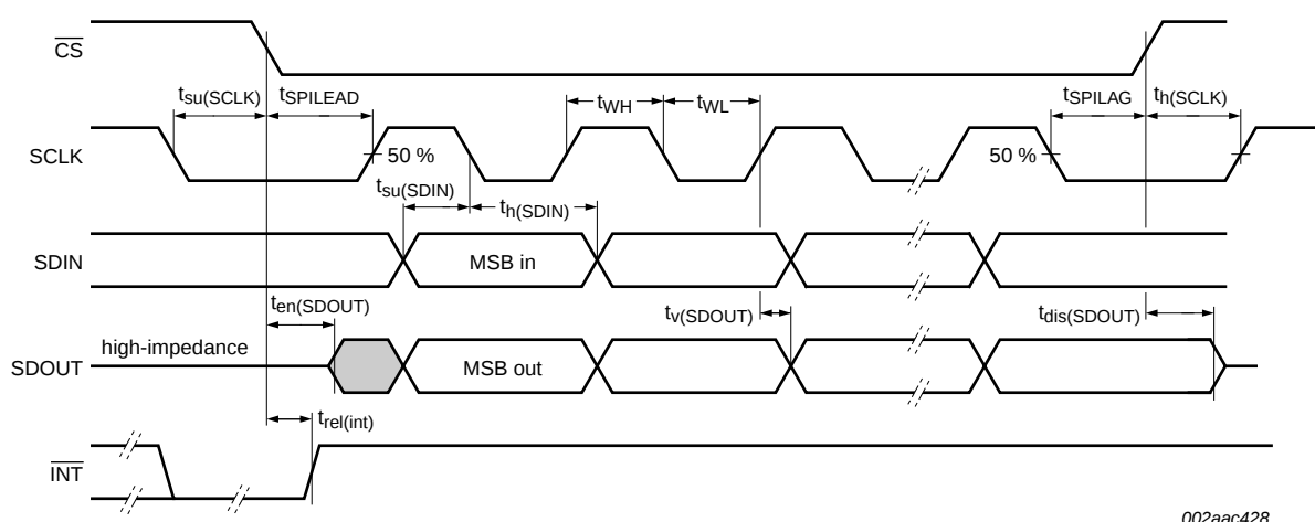
Fig 12. Timing diagram
