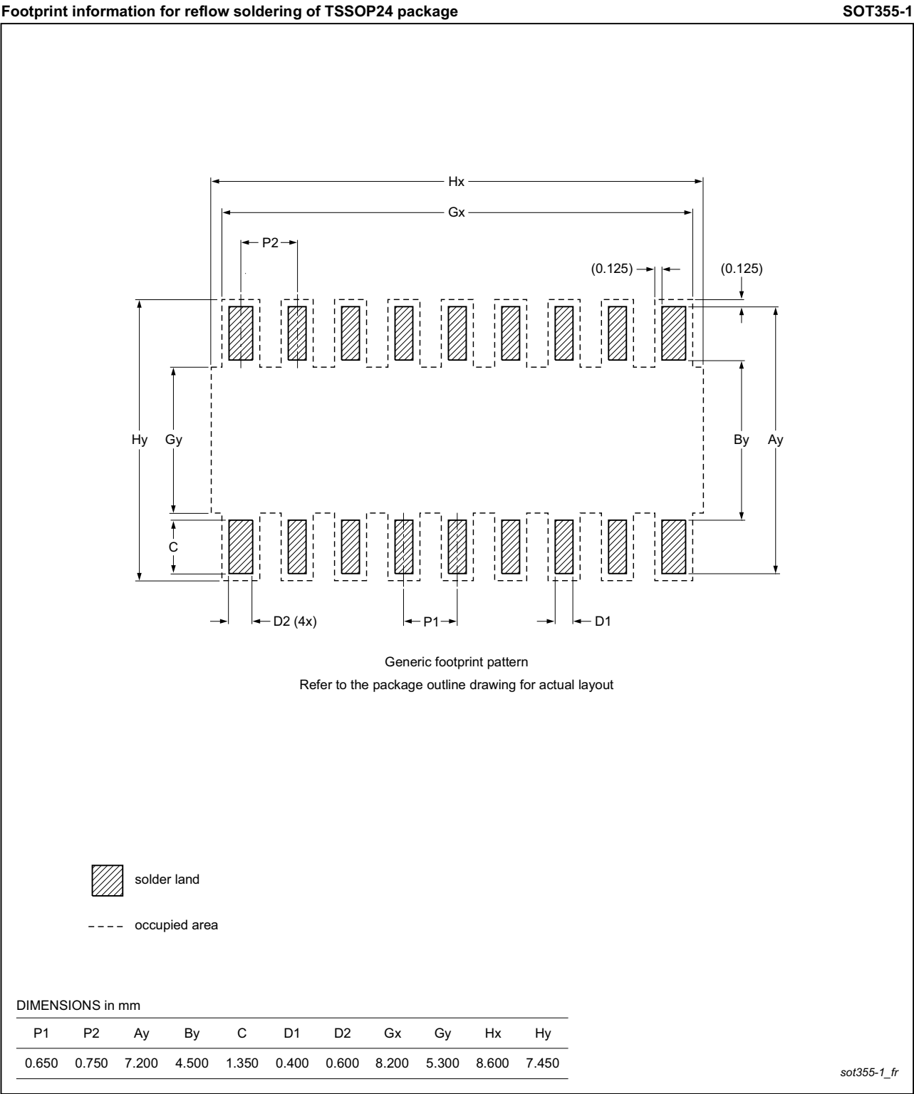
Fig 21. PCB footprint for SOT355-1 (TSSOP24); reflow soldering
