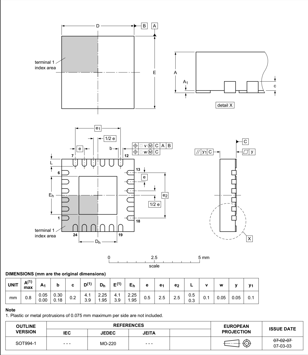
Fig 19. Package outline SOT994-1 (HWQFN24)
