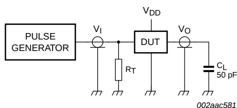
Fig 16. Test circuitry for switching times, SDOUT ( t_v(SDOUT) )
