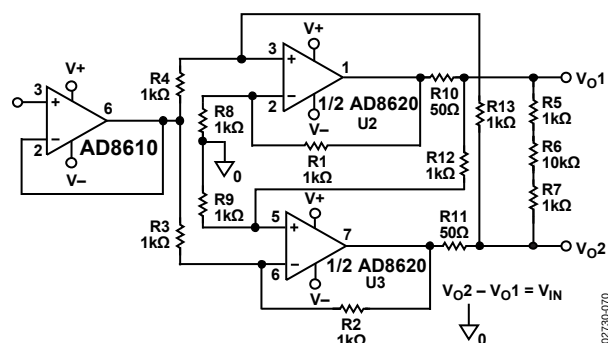
Figure 70. Differential Driver
