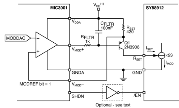
Figure 30. Controlling the SY88912
