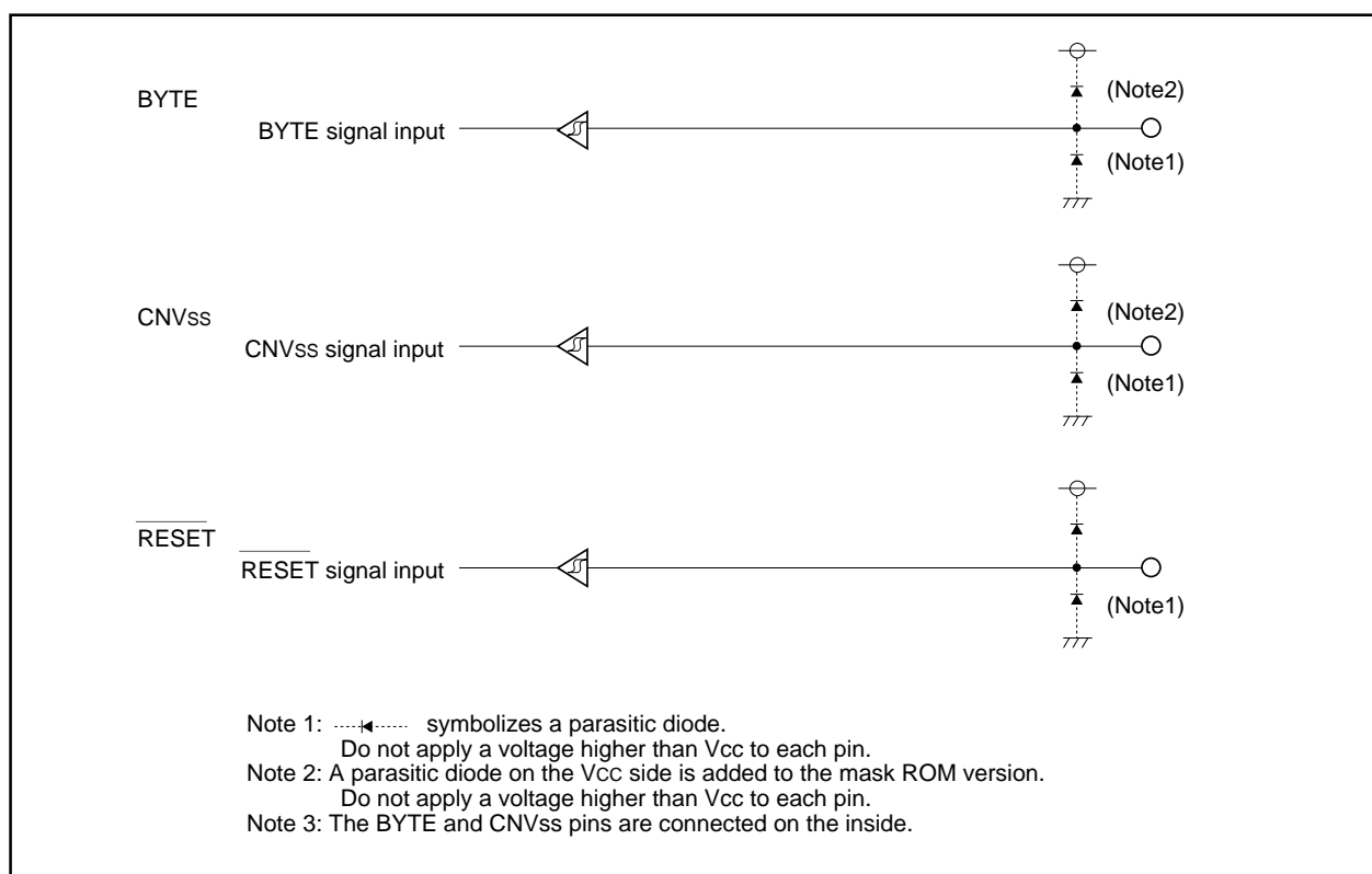
Figure 1.18.5. I/O pins
