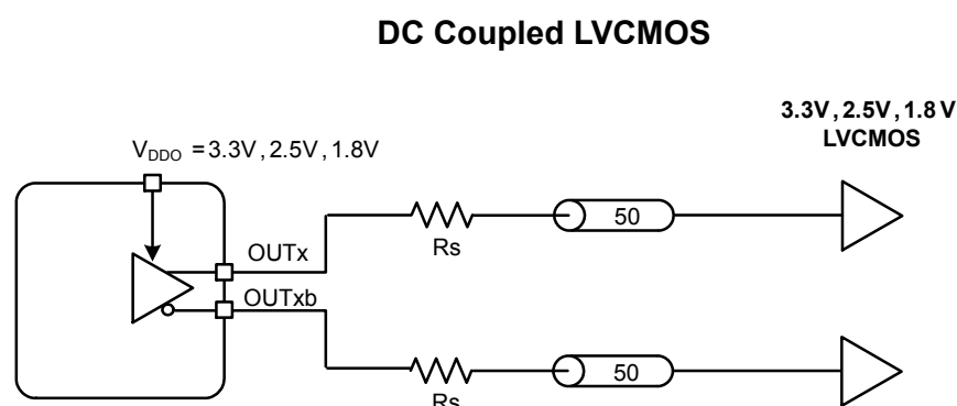
Figure 3.6. LVCMOS Output Terminations
