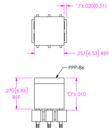
FIG 10 -P: PICK AND PLACE PAD (-03 POS ONLY) (DIFFERENT AS SHOWN, OTHERWISE SAME AS FIG 1) "J" = ((NO OF POS x .100 [2.54]) - .257 [6.53]) / 2
