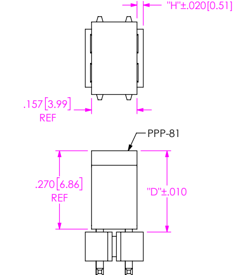
FIG 9 -P: PICK AND PLACE PAD (-02 POS ONLY) (DIFFERENT AS SHOWN, OTHERWISE SAME AS FIG 1) "H" = ((NO OF POS x .100 [2.54]) - .157 [3.99]) / 2
