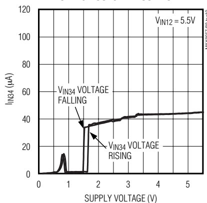
NO-LOAD SUPPLY CURRENT vs. SUPPLY VOLTAGE OUT3 AND OUT4 ONLY
