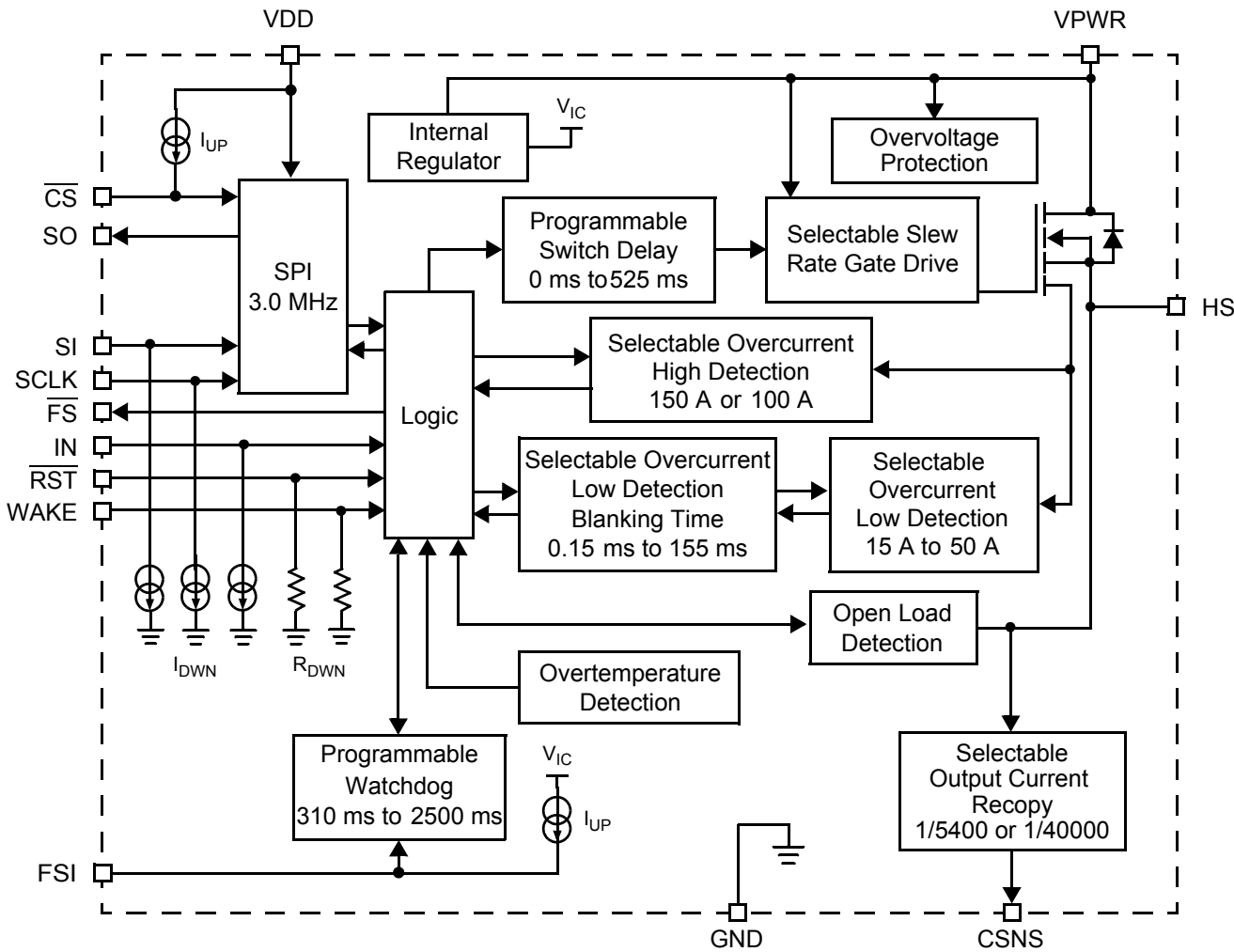
Figure 2. 33982 Simplified Internal Block Diagram
