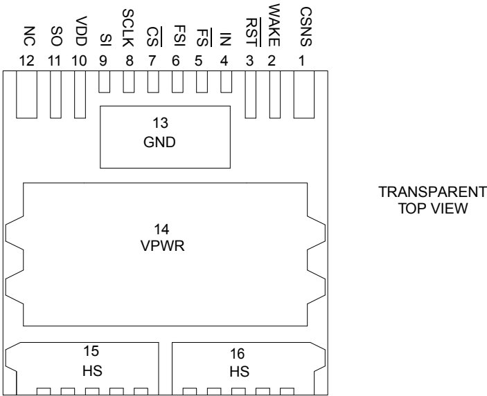
Figure 3. 33982 Pin Connections
