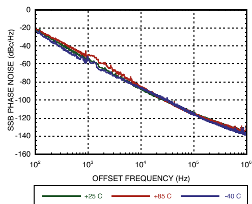
SSB Phase Noise @ V_{\text{tune}} = +5\text{V}
