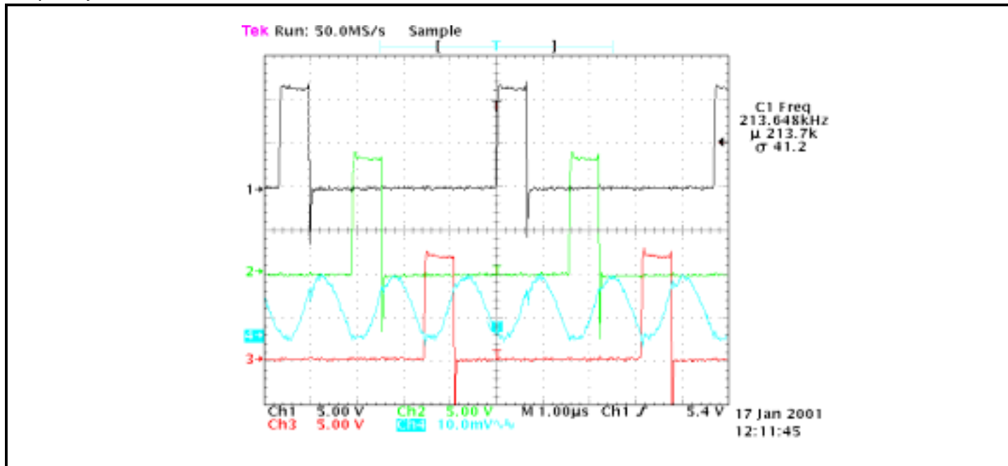
Fig. 11 - The typical phase node voltage and the output voltage ripple waveform under 60A full load operation.
