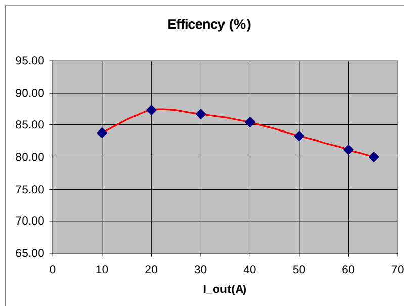
Fig. 10 - Typical efficiency curve for 12 mOhm top FETs and 4 Ohm bottom FETs.
