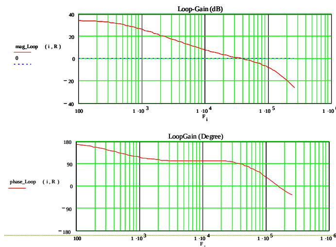
Fig. 5 - Loop gain Bode plot based on control loop model.
