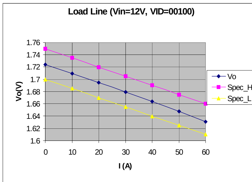
Fig. 9 - Measured output drooping characteristics of the 60A design.
