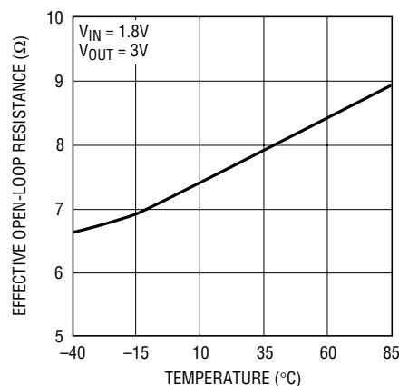
Figure 2. Typical R_{OL} vs Temperature
