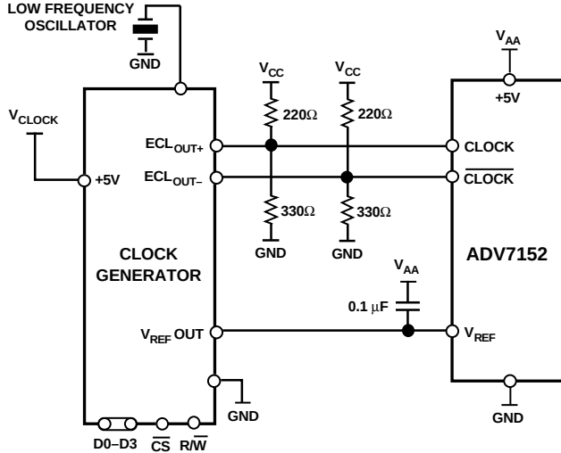
Figure 13. PLL Generator Driving CLOCK, \overline{\text{CLOCK}} of the ADV7152
