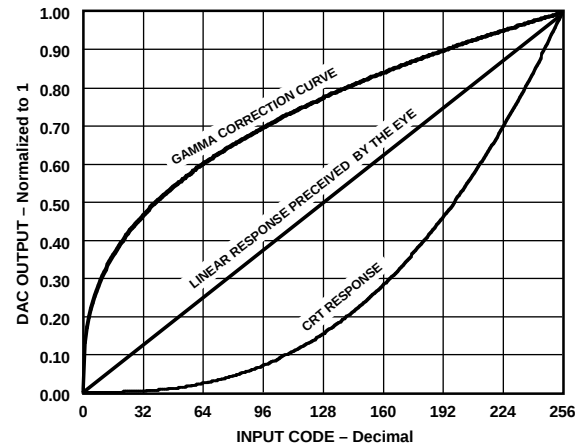
Gamma Correction Curve (Gamma Value = 2.7)
