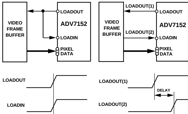
Figure 14. LOADOUT vs. Pixel Clock Input (CLOCK, \overline{\text{CLOCK}} )
