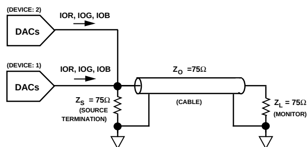
Multiple Devices Termination for a Single Monitor
