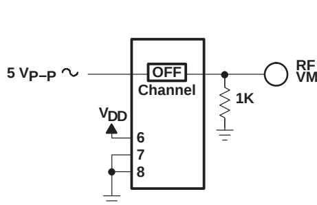
Figure 20. Feedthrough
