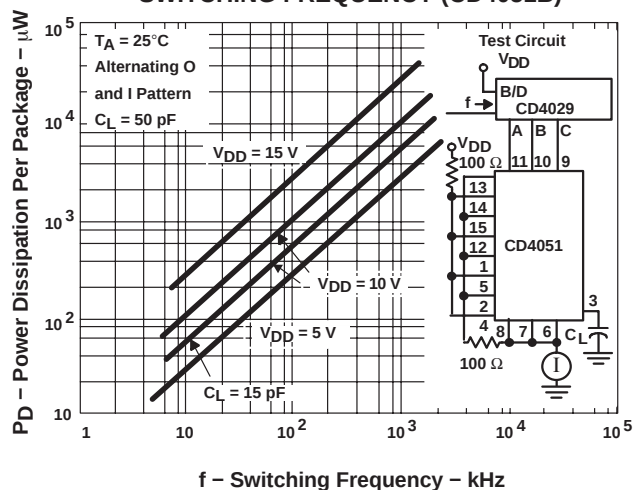
DYNAMIC POWER DISSIPATION VS SWITCHING FREQUENCY (CD4051B)
