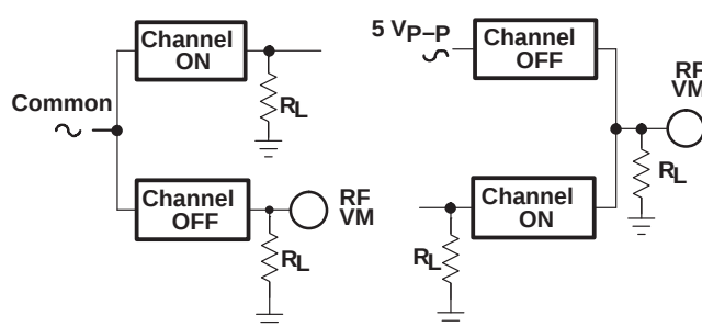
Figure 21. Crosstalk Between Any Two Channels
