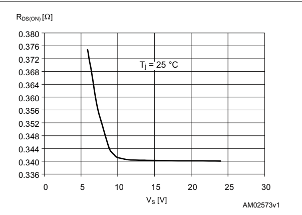
Figure 22. Typical high-side R_{DS(on)} vs. supply voltage
