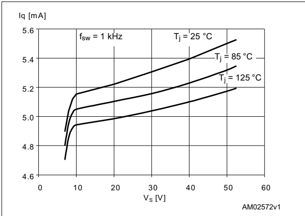
Figure 21. Typical quiescent current vs. supply voltage
