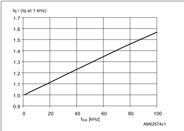
Figure 23. Normalized typical quiescent current vs. switching frequency
