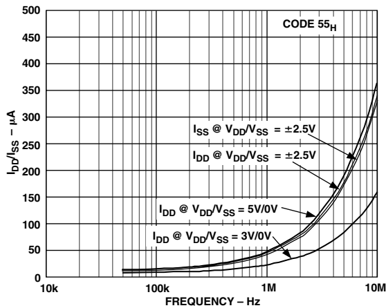
TPC 14. AD5200 10 kΩ Supply Current vs. Clock Frequency
