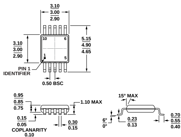
COMPLIANT TO JEDEC STANDARDS MO-187-BA Figure 15. 10-Lead Mini Small Outline Package [MSOP] (RM-10)
