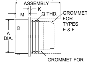
CRIMP KPSE00/MS3120
