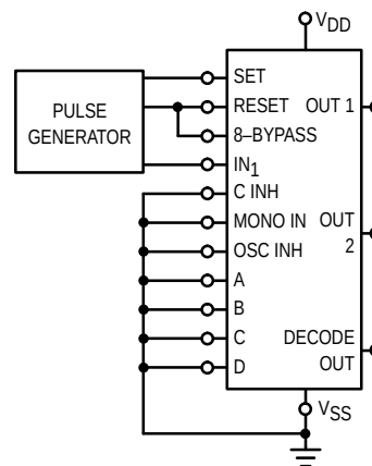
Figure 8. Functional Test Circuit
