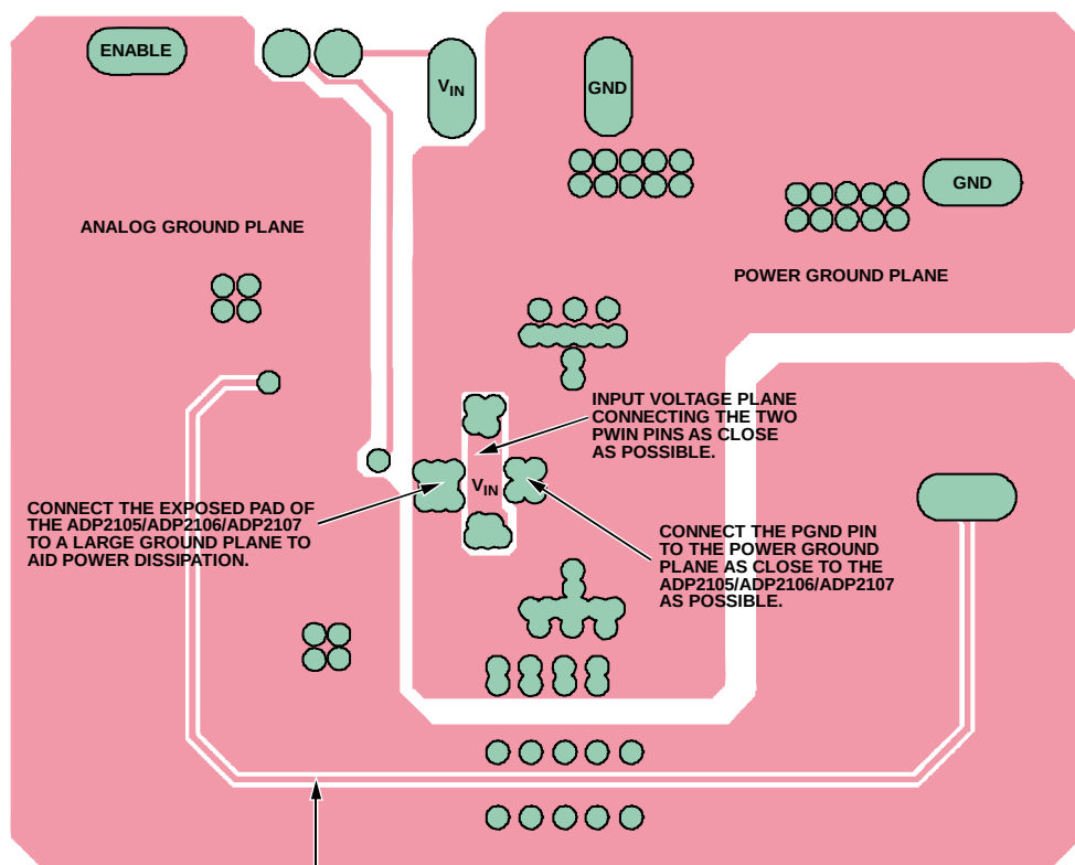
Figure 55. Recommended Layout of Bottom Layer of ADP2105/ADP2106/ADP2107
