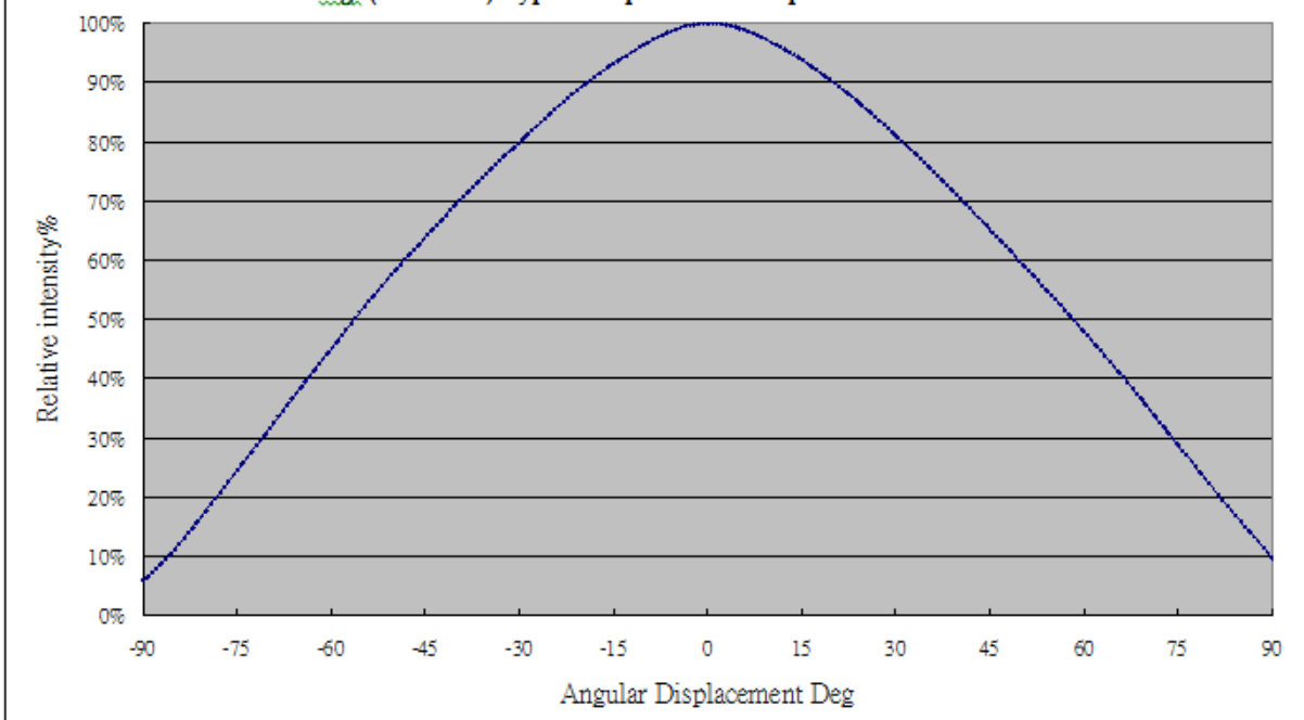
Fig. (120° Lens) Typical Representative Spatial Radiation Pattern
