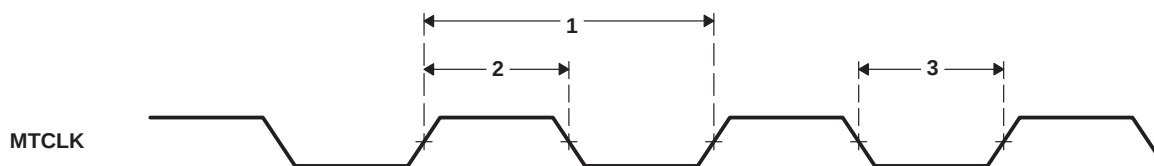
Figure 4–64. MTCLK Timing (EMAC – Transmit)
