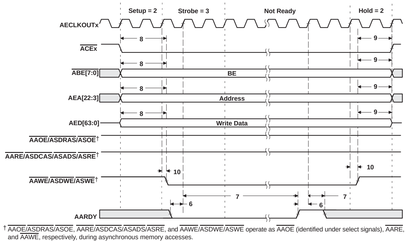
Figure 4-18. Asynchronous Memory Write Timing for EMIFA
