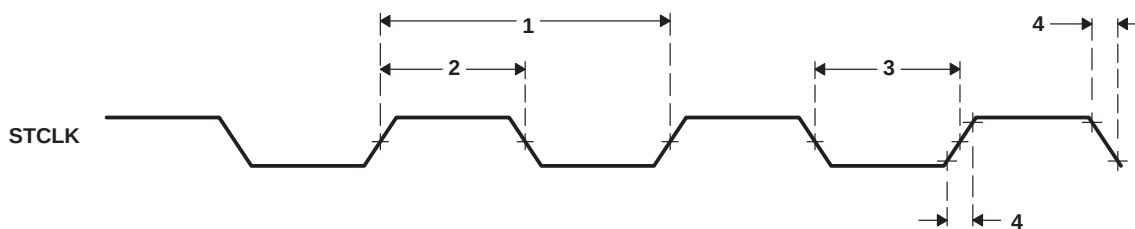
Figure 4–62. STCLK Timing
