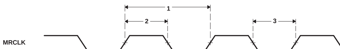
Figure 4–63. MRCLK Timing (EMAC – Receive)
