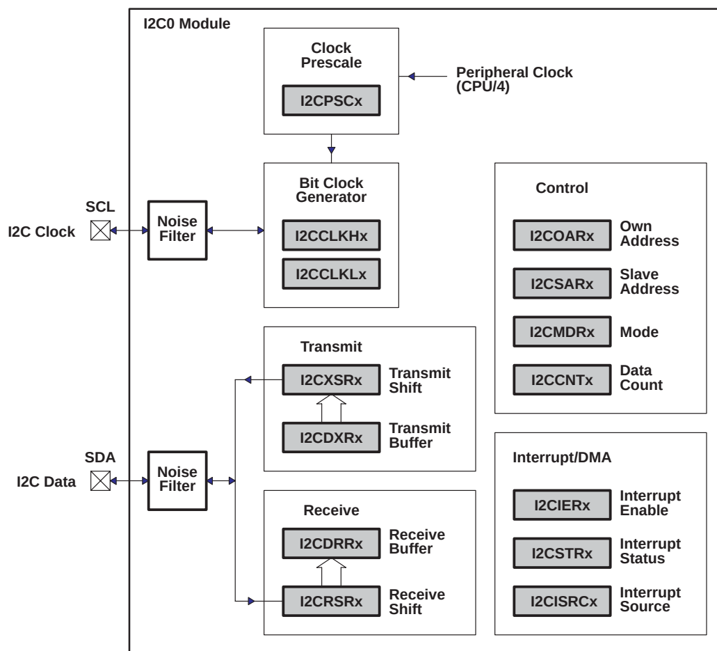
Figure 4–35. I2C0 Module Block Diagram
