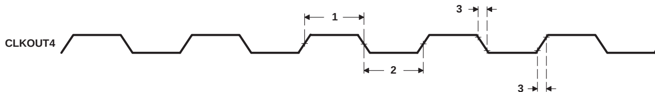
Figure 4-12. CLKOUT4 Timing
