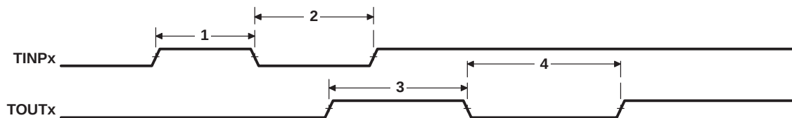
Figure 4–69. Timer Timing
