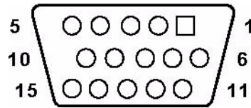
Figure 2.6 VGA Connector
