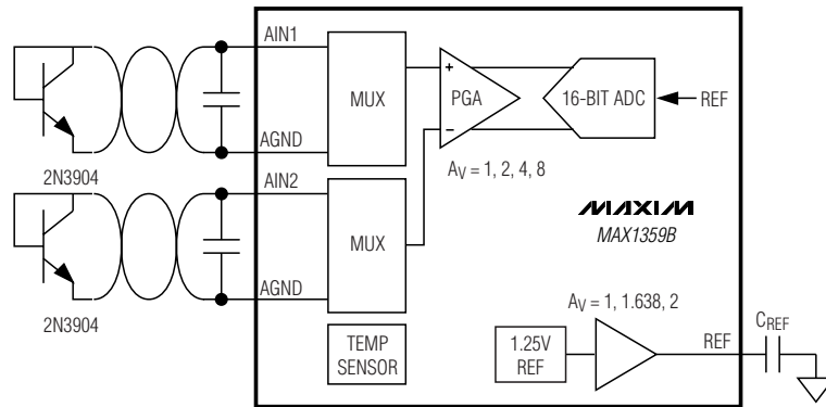
Figure 26. Temperature Measurement with Two Remote Sensors
