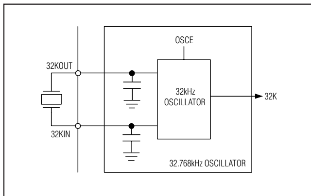
Figure 9. 32kHz Crystal-Oscillator Block Diagram
