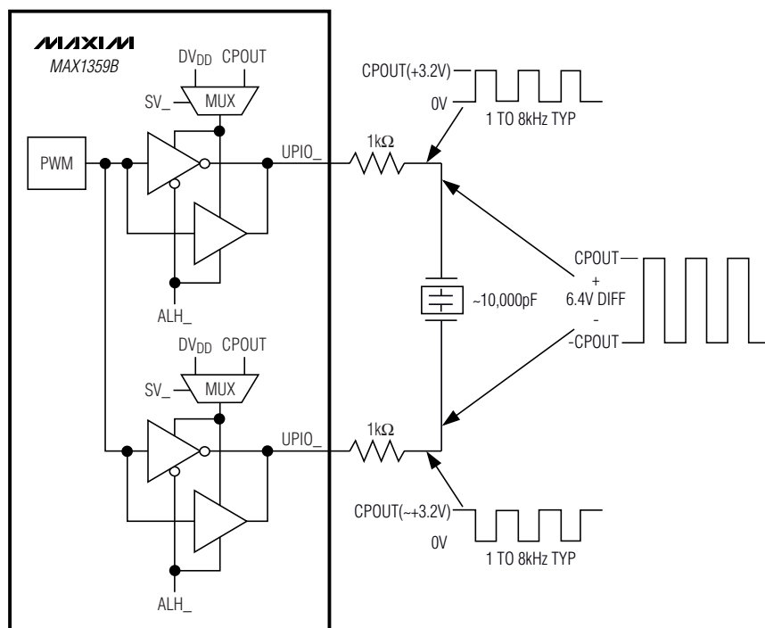
Figure 31. Differential Piezoelectric Buzzer Drive
