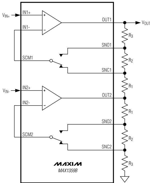
Figure 27. Programmable-Gain Instrumentation Amplifier
