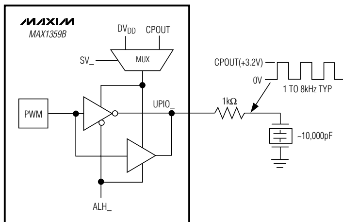
Figure 30. Single-Ended Piezoelectric Buzzer Drive
