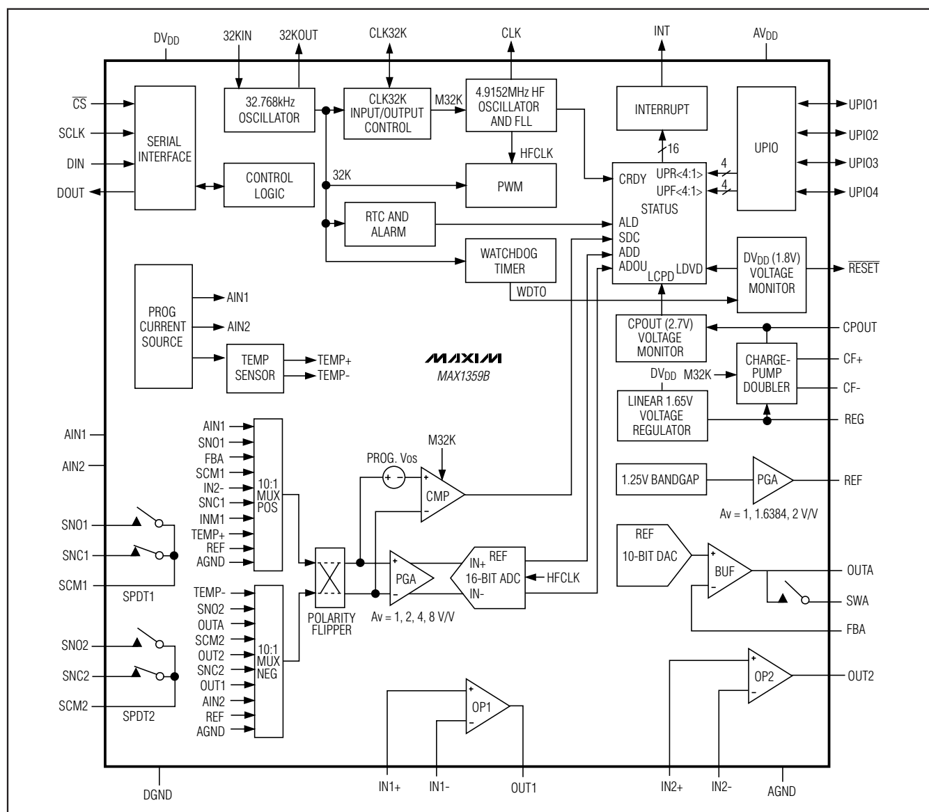
Figure 3. Functional Diagram
