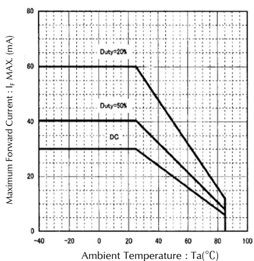
Derating Ambient Temperature vs. Maximum Forward Current Repetition Frequency : f \geq 100\text{Hz}
