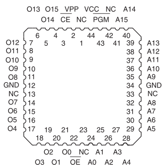
PLCC Top View
